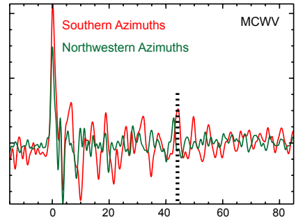
Averaged Receiver Functions
